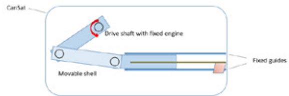
Figure 2: Deployment system scheme
