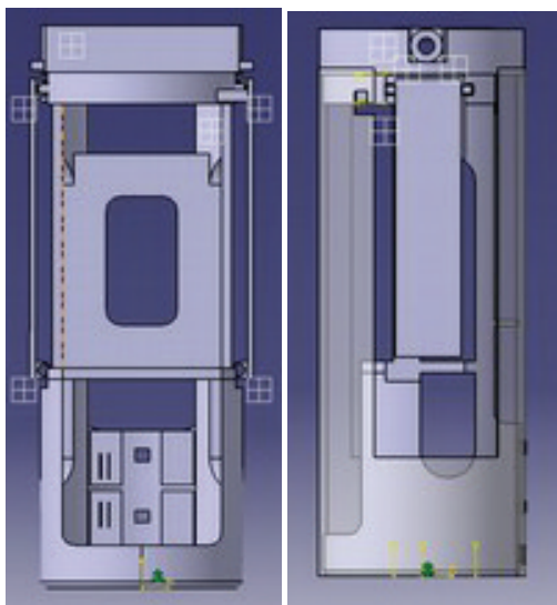
Fig 8: Front and lateral view of the structure
