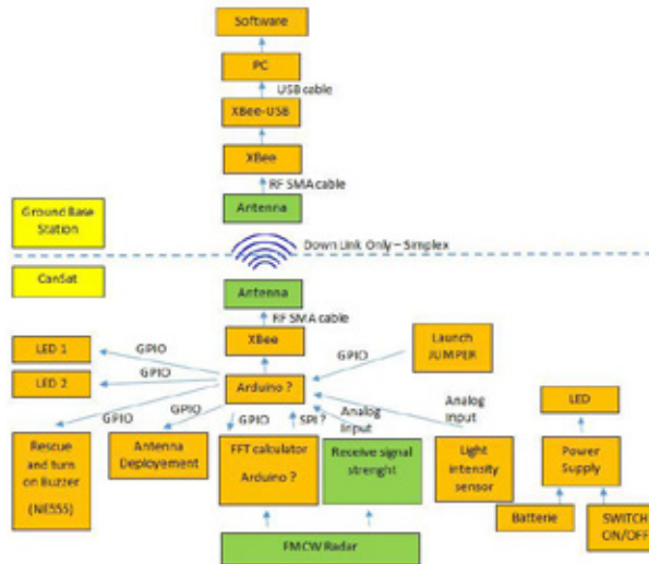
Fig. 3. CanSat Architecture.
