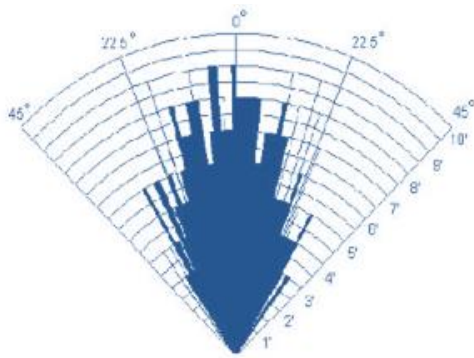
Figure 7 : Ultrasonic angular performance
