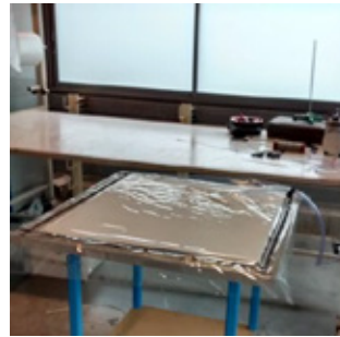
Figure 6 : Carbon fiber in vacuum bag
