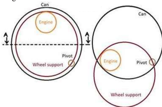
Fig3. Side view of the rover, and wheels dropping system
