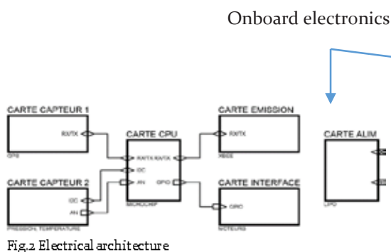
Fig.2 Electrical architecture
