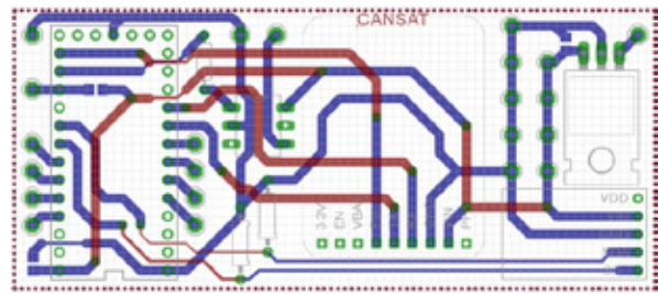
Fig. 2. Main board typon
