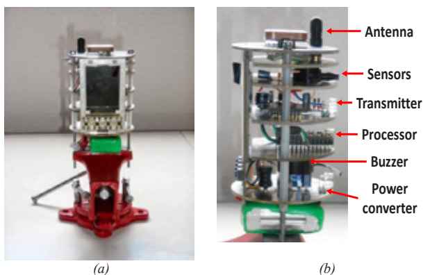
Fig. 2. EirSpace international class CanSat launched in august 2014. (a) Front view. (b) Side view.
