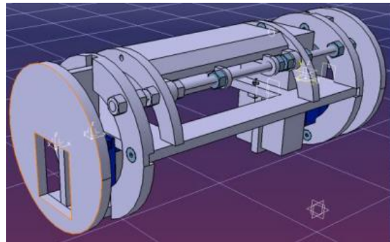
Fig. 3. CAD Model of the CanSat
