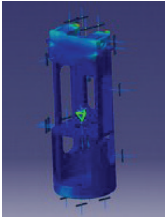
Fig 12: visualisation of the stress over the structure
