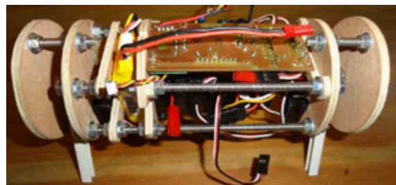
Fig. 4. Final CanSat structure
