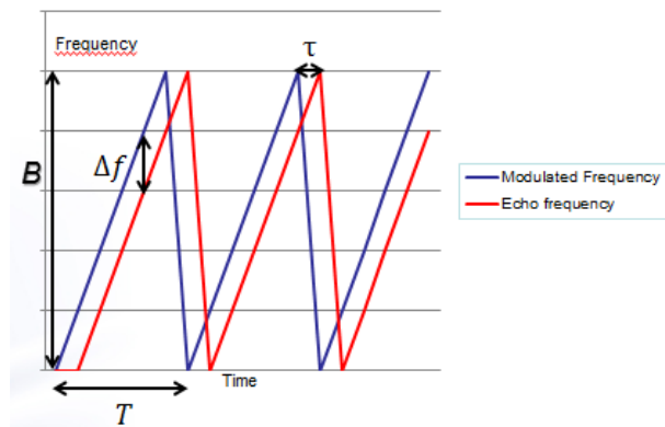
Fig. 4. Triangular frequency modulated profile.
